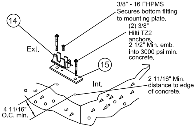
Anchor detail
